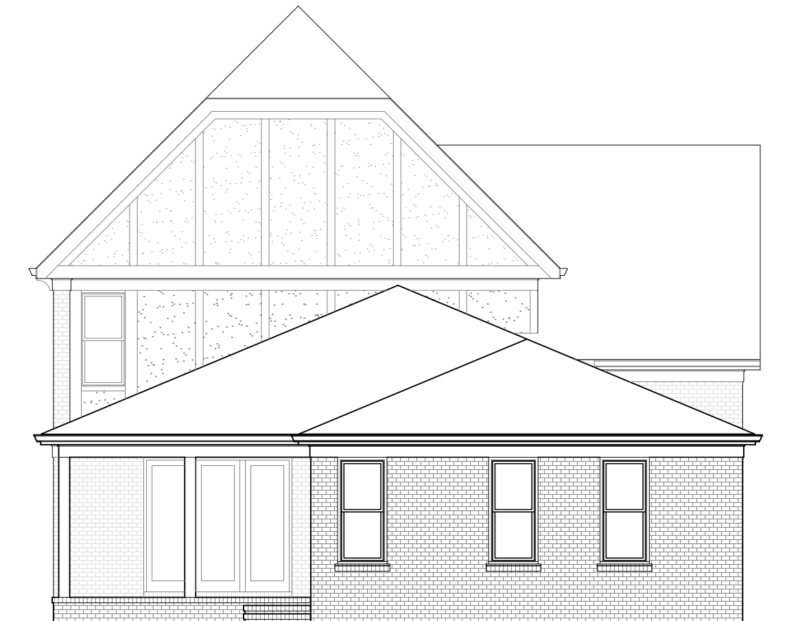
REAR ELEVATION
