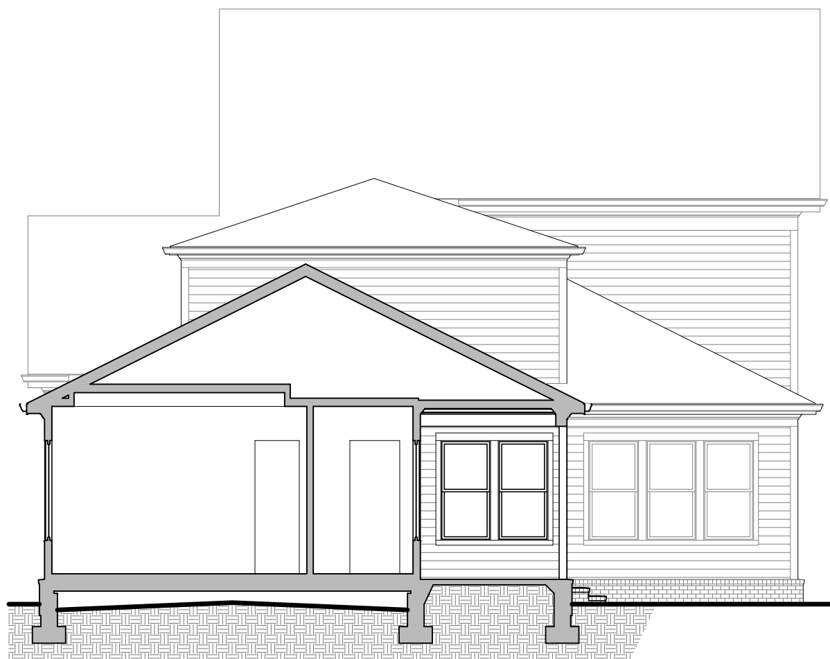
AUXILIARY REAR ELEVATION
